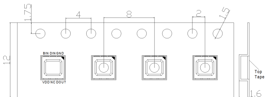
Carrier tape specifications (unit: mm)
